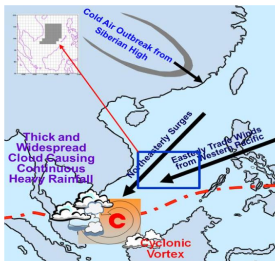
Effects of the northeast monsoon on rainfall
