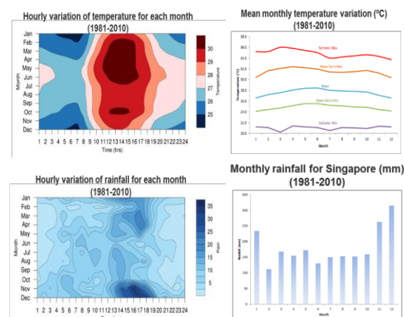
Temperature and rainfall variations in Singapore
