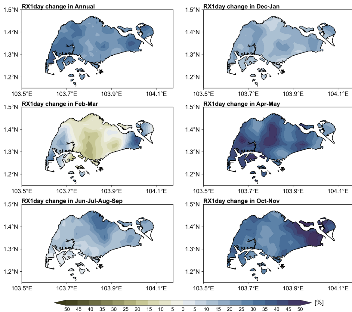
Figure 5.3: Percentage change in daily maximum rainfall annually, in December–January, February–March, April–May, June–July–August–September, and October–November months, during end-century (2080–2099) period relative to the baseline (1995–2014) under the high emissions scenario.
