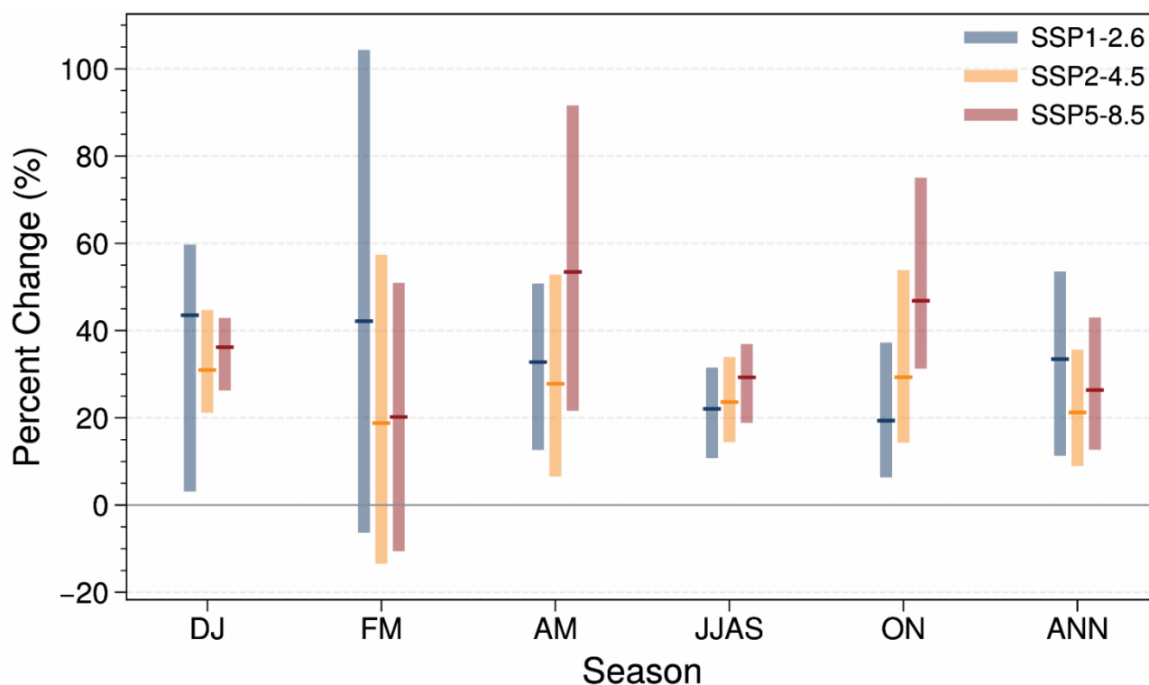
Figure 5.4: Projected changes in very heavy daily rainfall annually, and for each of the seasons during the end-century under the three SSP scenarios.
