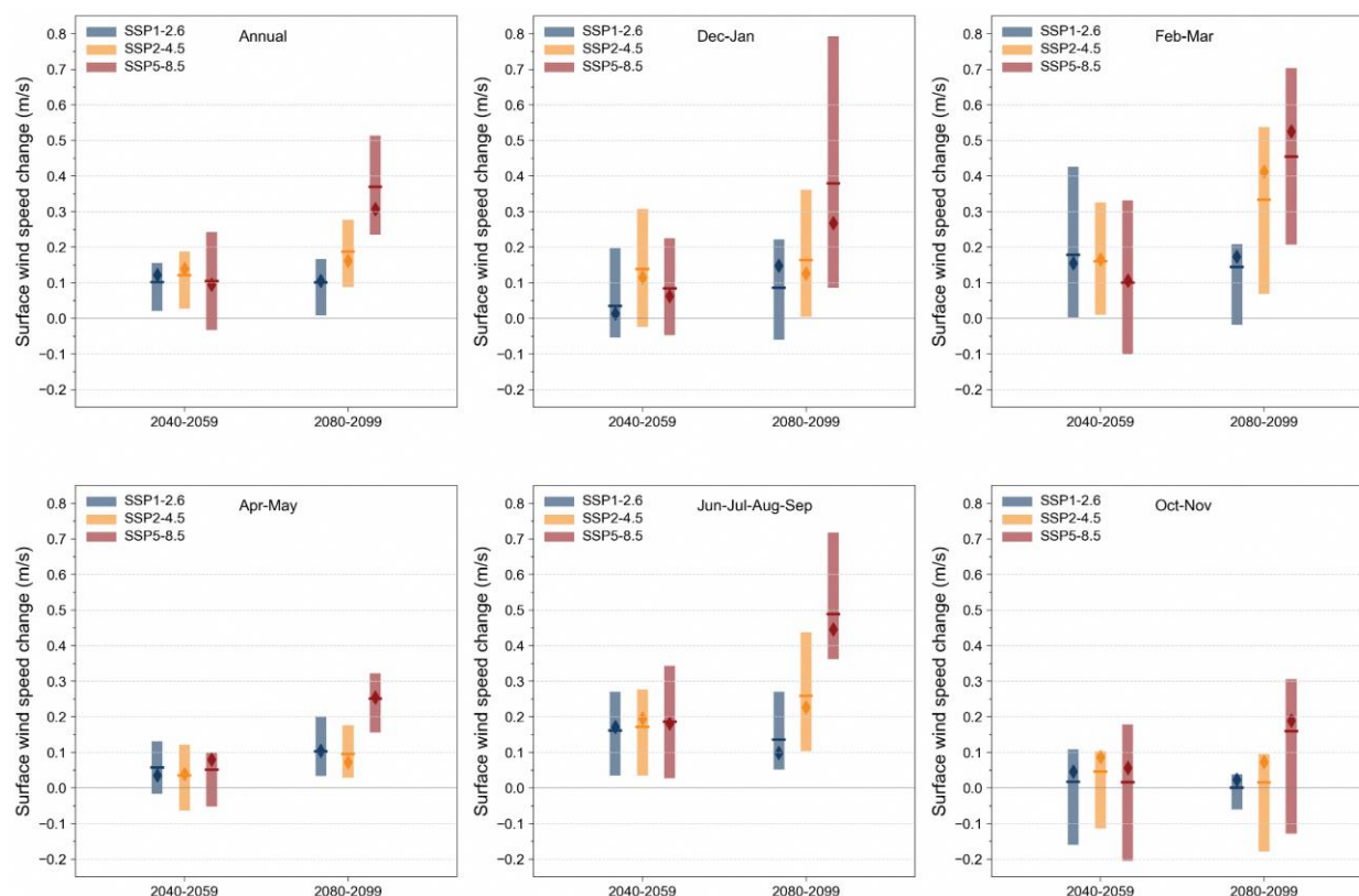
Figure 10.15: Changes in mean 10m wind speed for annual, December–January, February–March, April–May, June–July–August–September, and October–November during mid- (2040–2059) and end-century (2080–2099) periods for the 5 bias-adjusted downscaled GCMs (2 km) over Singapore relative to the baseline (1995–2014). The line and thin diamond represent the mean and median over the 5 models, respectively. For readability, the values are available in Tables 10.41–10.46.
