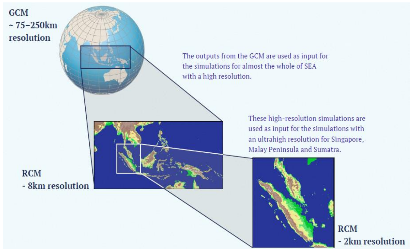
Figure 2.3: The dynamical downscaling design for V3.
