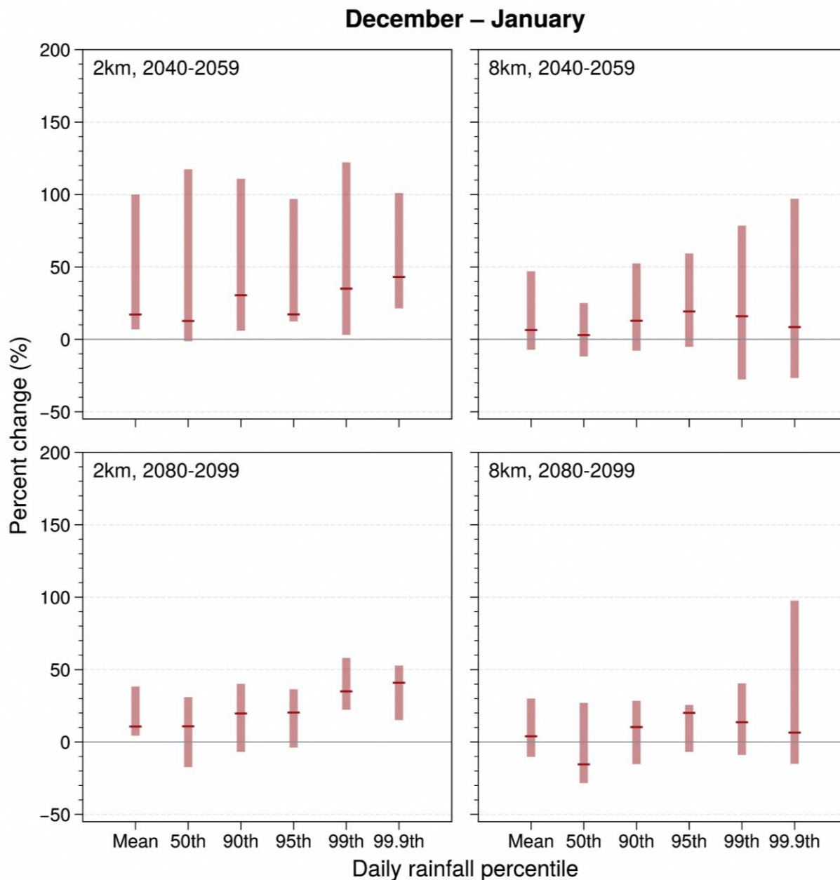
Fig A10.3: Changes in Singapore average daily rainfall amount during December - January (wet phase of NE monsoon) for the mid-century (2040-2059; top row) and end-century (2080-2099; bottom row) periods from SINGV-RCM downscaled simulations at 2-km (left) and 8-km (right). Shown are the percentage changes in the mean and at different percentiles (50th, 90th, 95th, 99th and 99.9th) under the SSP5-8.5 scenario. The mean and percentile values are derived only from wet days (rainfall \geq 1mm/day); each percentile uses the nearest corresponding daily rainfall value.
