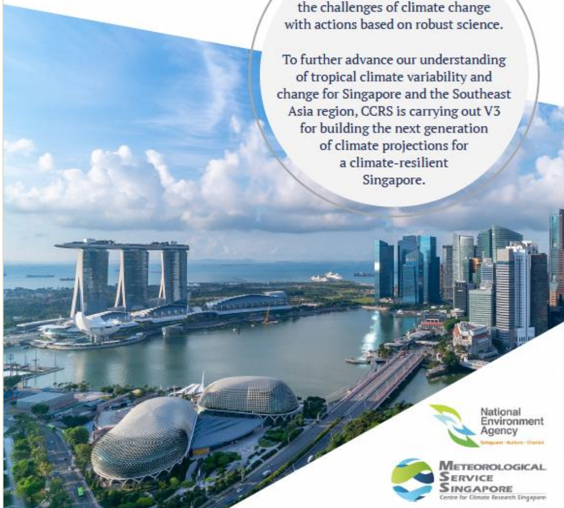
Figure 14.1: Cover page of the 'V3 Explained' brochure
