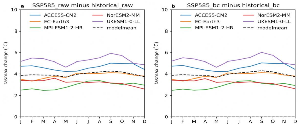
Figure 9.13: Changes in the Singapore domain-averaged tasmax from the historical period (1995-2014) to the future period (2080-2099) under the SSP585 scenario. a. raw simulations. b. bias-adjusted simulations.
