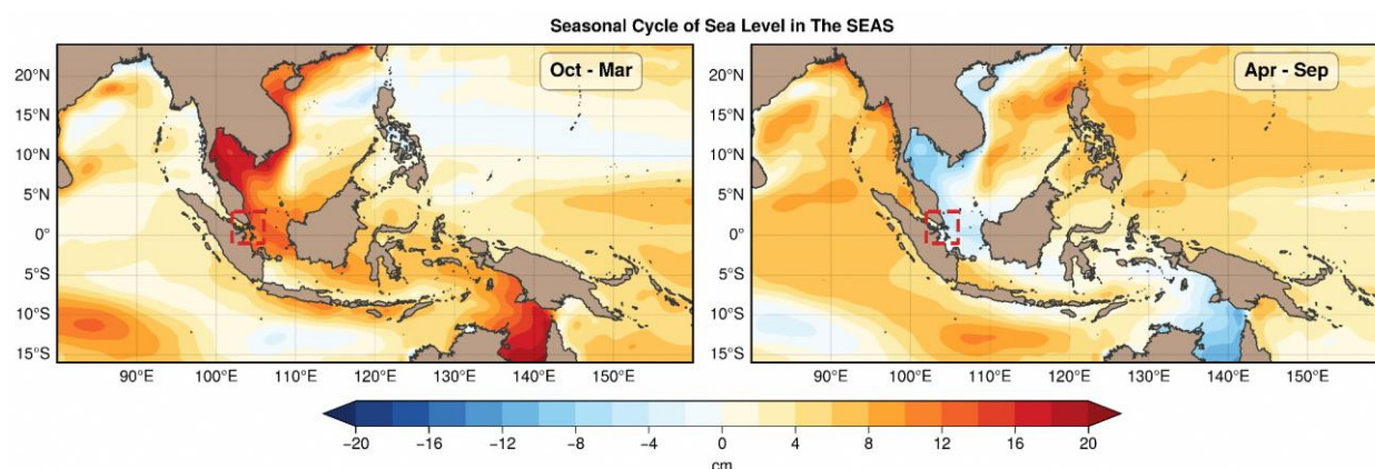
Figure A12.1: Seasonal cycle of sea level in the southeast Asian seas computed from satellite data for the period 1993 - 2021.
