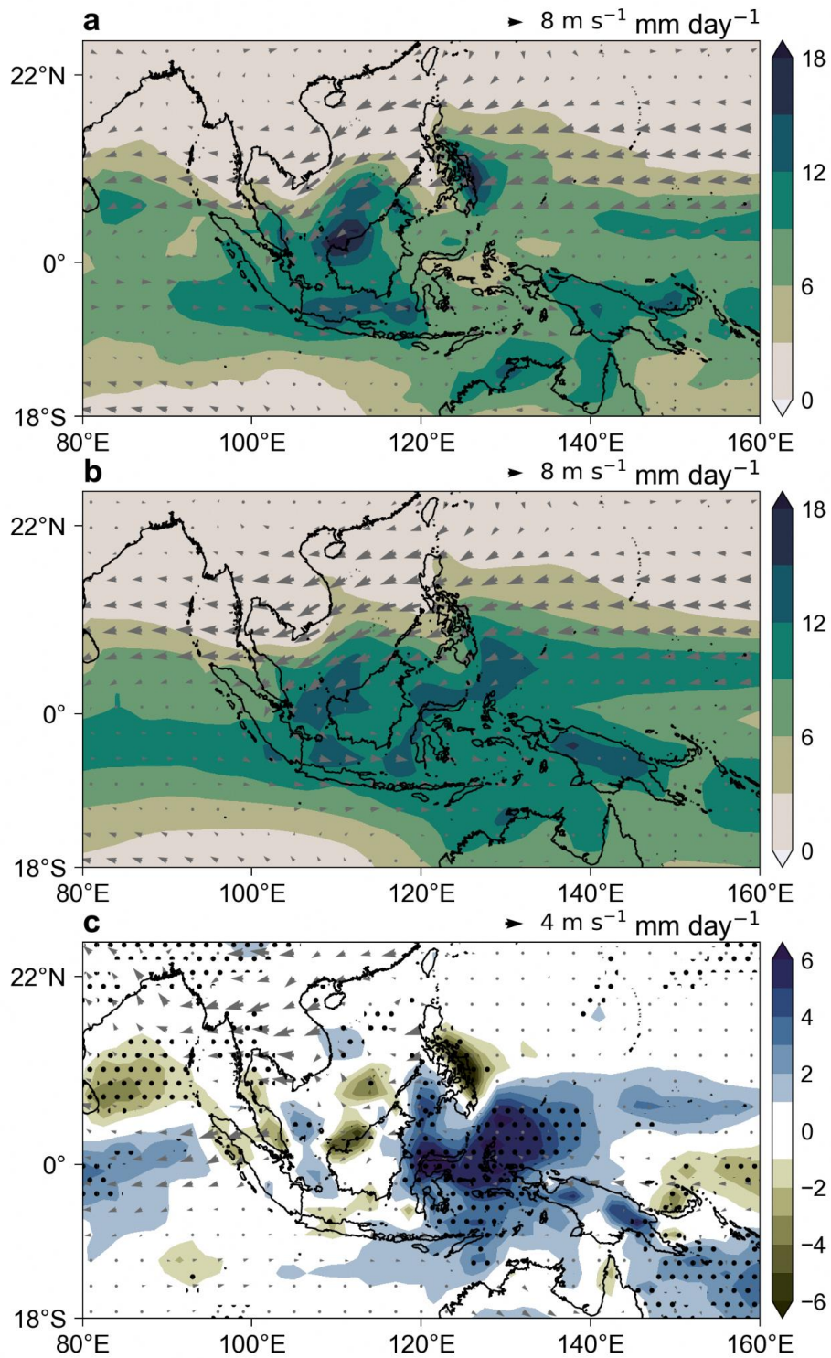
Figure 5.24: (a) Precipitation and 850 hPa winds composited over surge days in REF (winds and PSL are derived from the ensemble mean of ERA5, MERRA2, and JRA55, precipitation the ensemble mean of 5 datasets from FROGs: CMORPH, GSMAP, IMERG, PERSIANN-CDR, and TRMM 3B42). (b) As in (a), but for 36 CMIP6 models. (c) Model bias in surge precipitation and winds (i.e. (b) - (a)).
