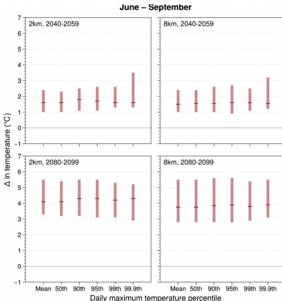
Figure A10.11: As in Figure A10.8 but for June - September (SW monsoon period).
