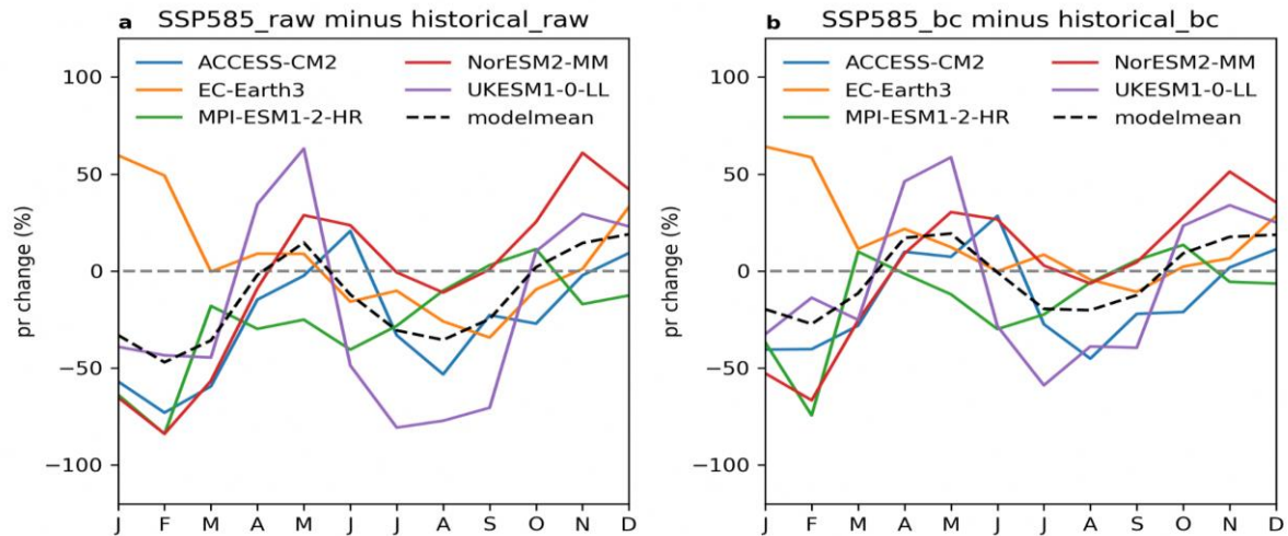
Figure 9.27: Percentage changes in the Singapore domain-averaged pr from the historical period (1995-2014) to the future period (2080-2099) under the SSP585 scenario at a 2km resolution. a. raw simulations. b. bias-adjusted simulations.
