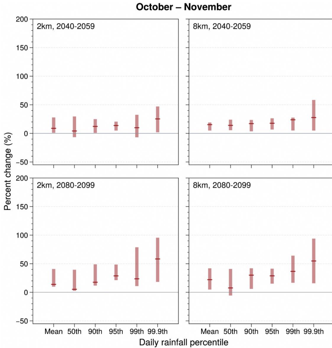
Figure A10.7: As in Figure A10.3 but for October-November (2nd intermonsoon)
