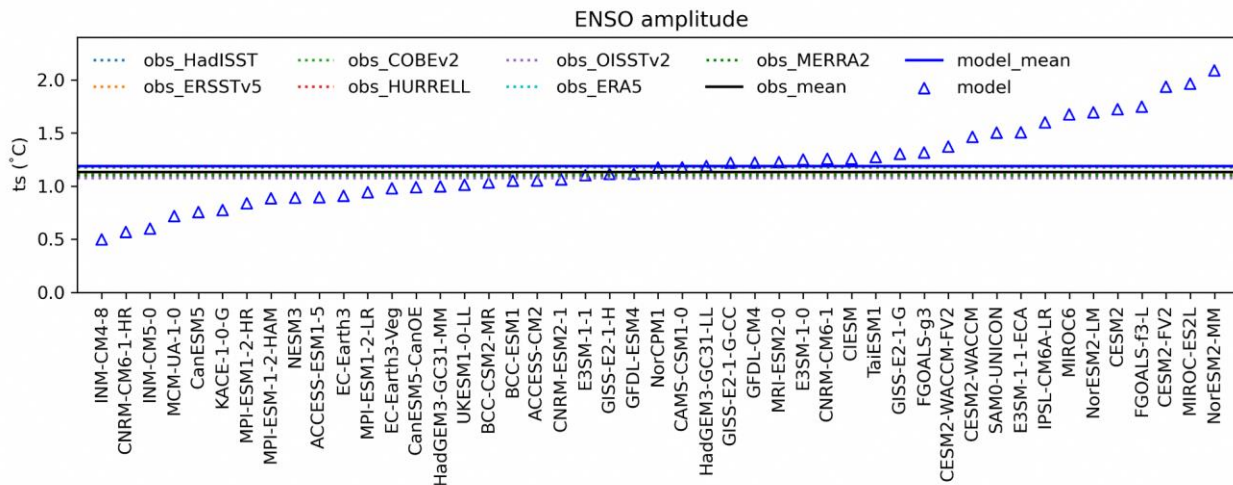
Figure 5.19: ENSO amplitude defined as standard deviation of Nino3.4 index (1985-2014 DJF mean).
