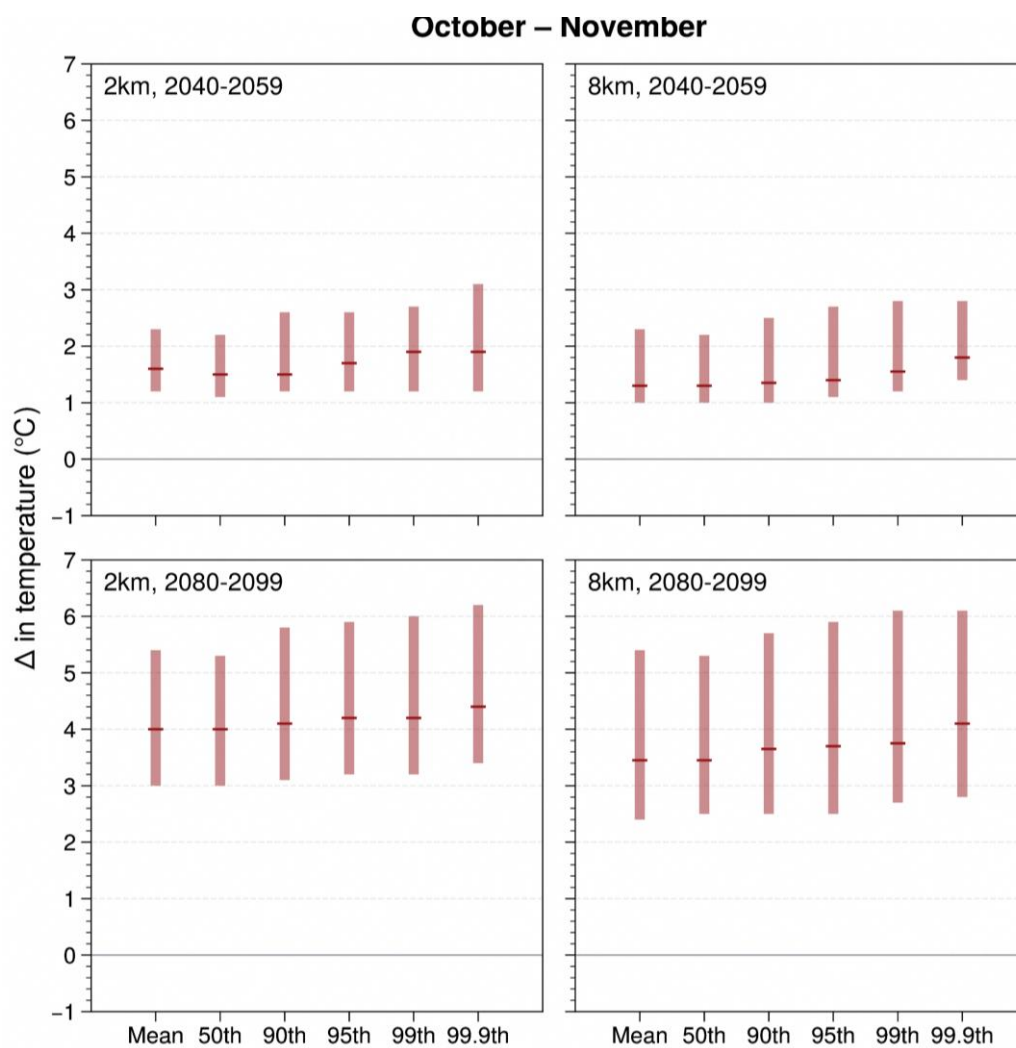
Figure A10.12: As in Figure A10.8 but for October-November (2nd intermonsoon)
