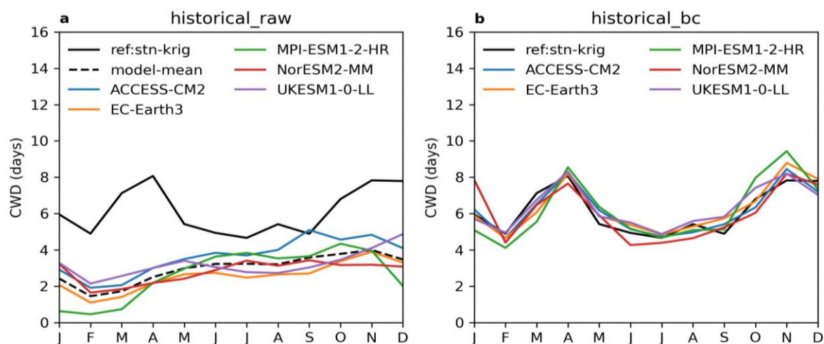
Figure 9.45: Singapore domain-averaged CWD in the historical period (1995-2014). a. observation reference (station krig pr) and raw simulations. b. similar to a, but plotting bias-adjusted simulations. Note that the value of CWD represents the wet days starting from individual month instead of truncated to the given month.
