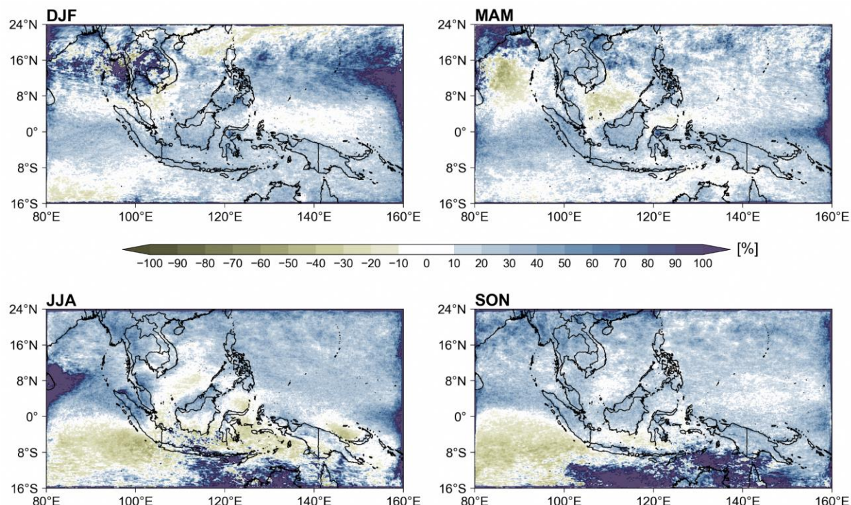
Figure 8.4: Percentage change of ensemble-mean downscaled (8km) changes in seasonal RX1day over end-century (2080-99) relative to the historical period (1995-2014) over the SEA domain under the SSP5-8.5 scenario.
