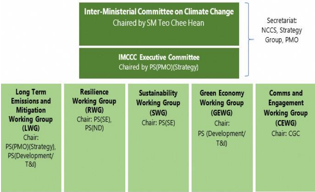
Figure 2.1: Climate Change Governance in Singapore (from NCCS, 2023).
