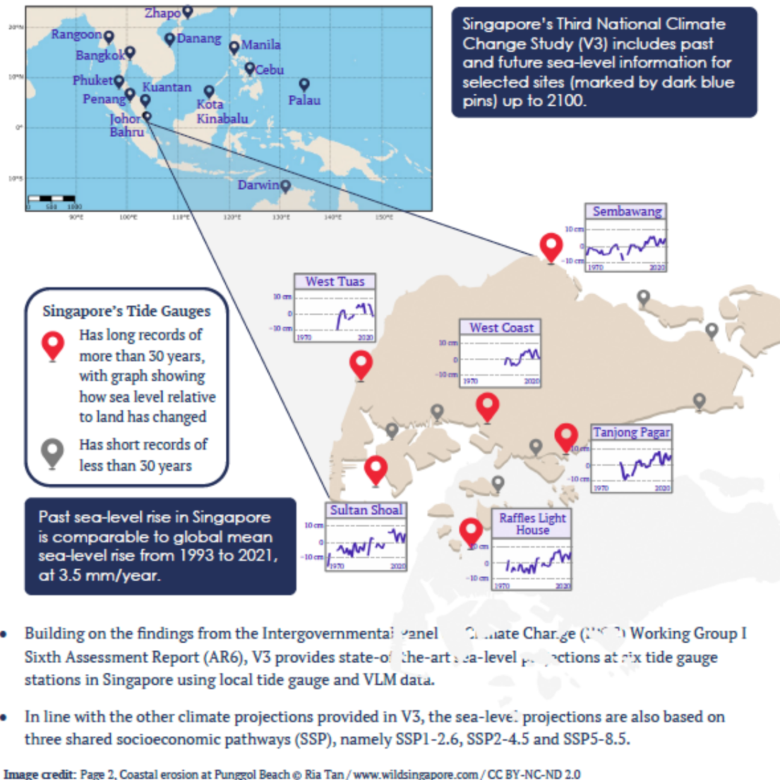
Figure 14.12: The 'Past and Future Sea-level Change' brochure presents the available past and future sea-level information from V3 for Singapore and the surrounding region.
