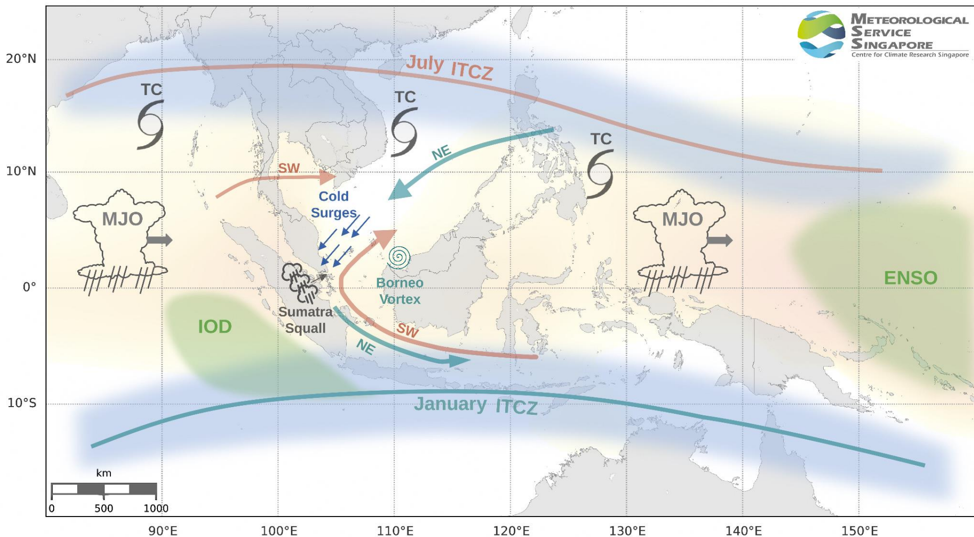
Figure 2.2: Climate drivers influencing weather and climate for the region around Singapore. Included are the average position of the Inter-tropical Convergence Zone (ITCZ) in blue indicating the furthest northward and southward extent of the seasonal migration of the regional monsoon system. The green and orange arrows indicate the corresponding Northeast and Southwest monsoonal flows. Against the background of warm ocean waters (soft orange colour indicating regions above 28.5°C), the El Niño–Southern Oscillation (ENSO) and Indian Ocean Dipole (IOD) impact the region's rainfall patterns on seasonal and inter-annual timescales, while the Madden-Julian Oscillation (MJO) impacts the region's rainfall at weekly to monthly timescales. At shorter timescales, Sumatra Squalls, Cold Surges and the Borneo Vortex can be sources of strong rainfall events. Further afar, tropical cyclones (TCs) can develop near the ITCZ away from the equator.
