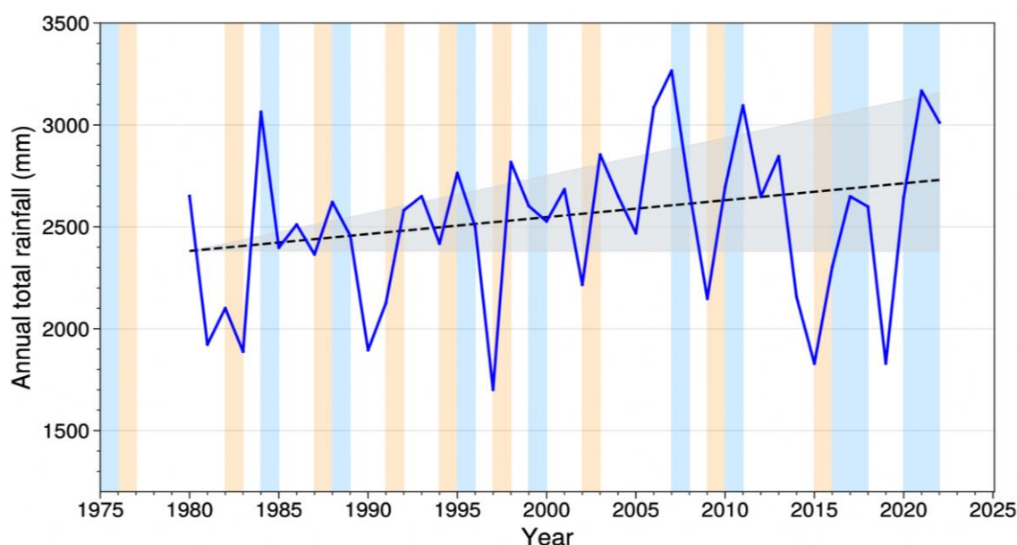
Figure 2.10: Annual total rainfall (solid blue) averaged over 32 stations with continuous records for at least 30 years. The black dashed line depicts an upward but not statistically significant trend (83 mm/decade). The grey shaded area represents the 95% confidence interval of the estimated trend.
