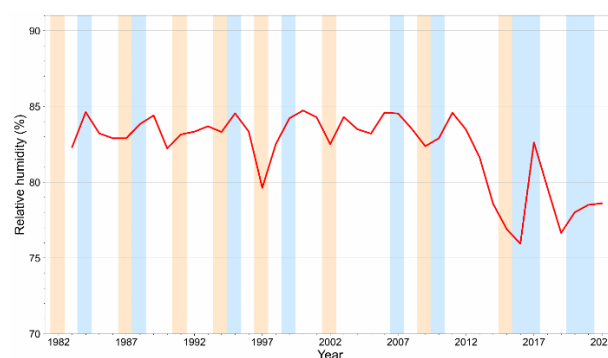
Figure 2.13: Annual mean relative humidity at Changi.
