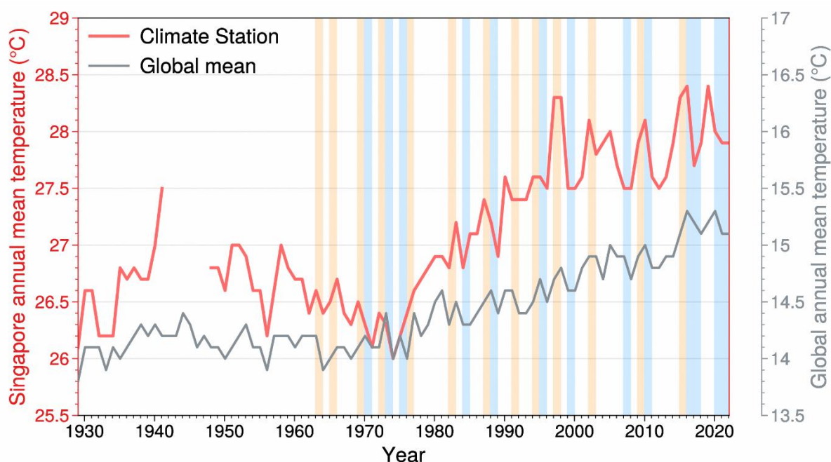
Figure 2.7: Annual mean temperature from 1929–2022 at Singapore's climate station, compared with the global annual mean temperature from the high-resolution ( 0.25^\circ \times 0.25^\circ ) Berkeley Earth dataset. The orange and blue bars denote El Niño and La Niña years from 1963, respectively.
